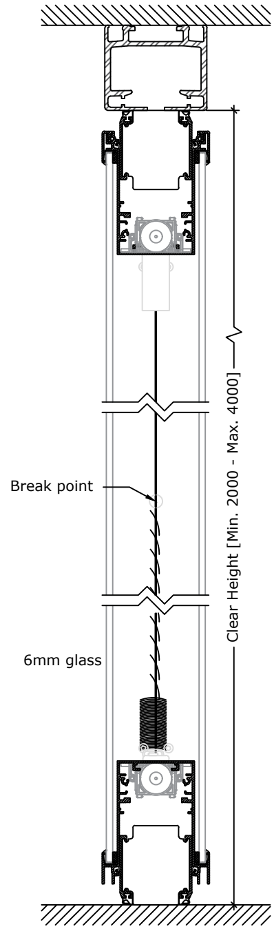
SECTION Scale 1:5
